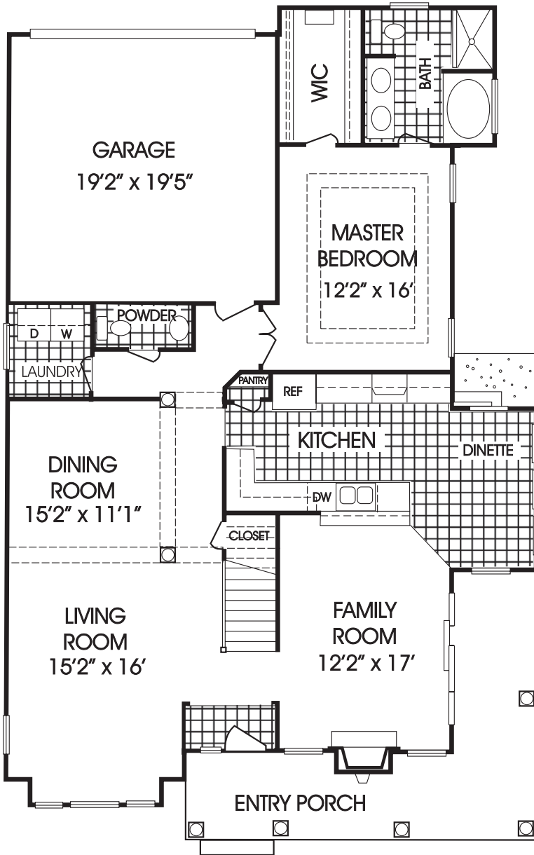
Plan A1080/1081 First Floor
