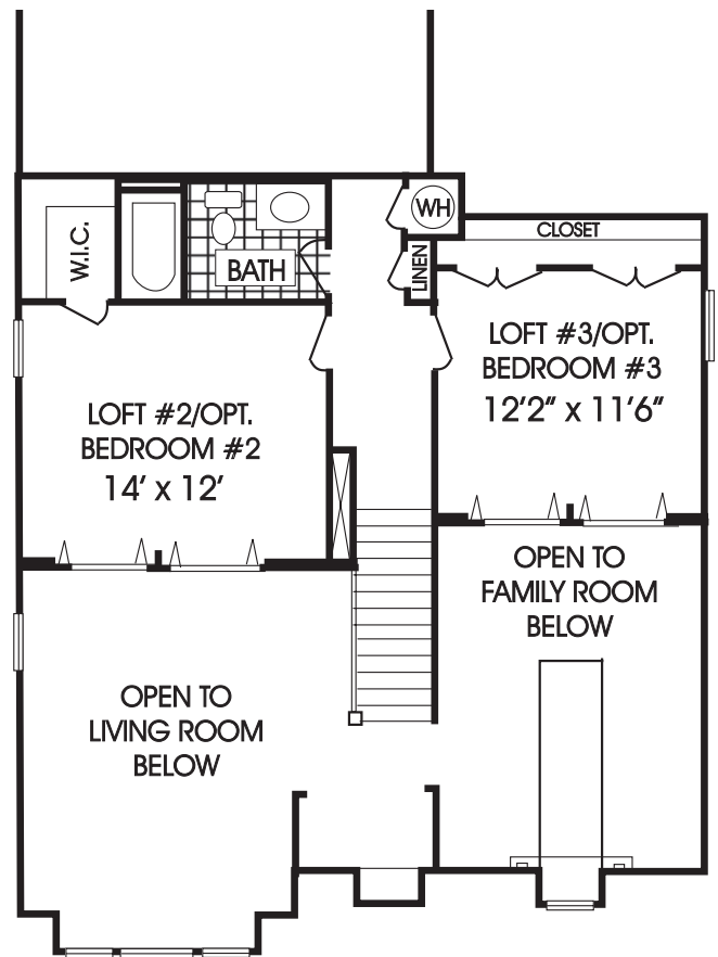
Plan A1080 Second Floor
